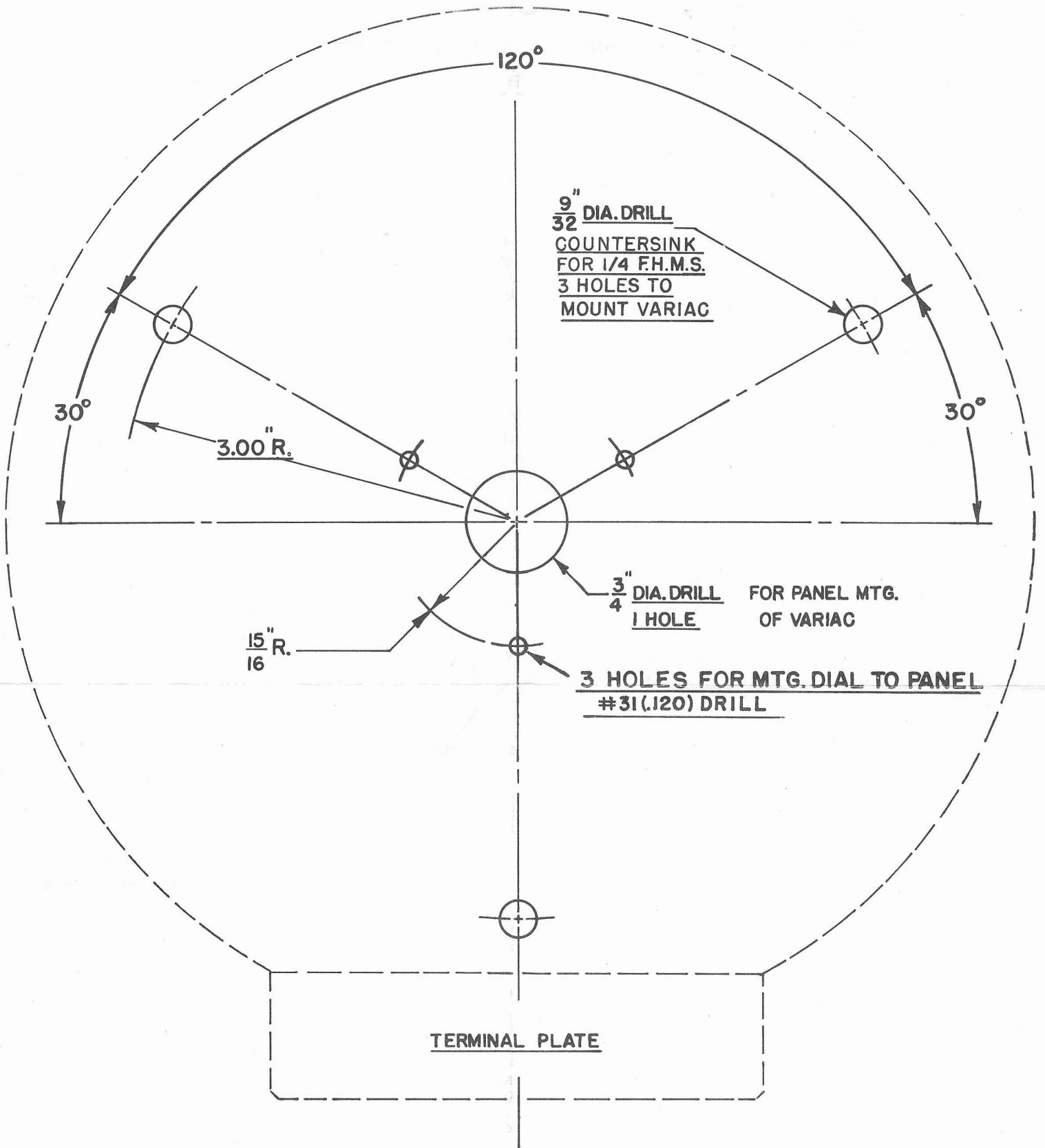
DRILLING TEMPLATE FOR V-20 VARIACS.
